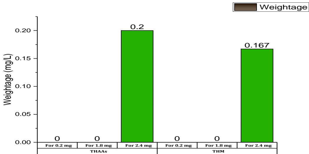
Figure 8. Founded THAAs and THMs for Different Chlorine Dosages
