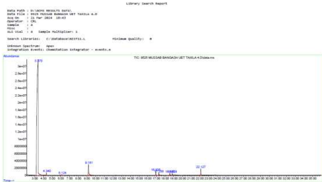
Figure 7. Obtained Mass Spectrometry for traced DBPs for Zone 3 Water Sample
